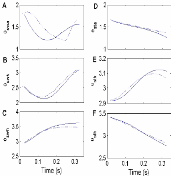
Figure 6. Simulation joint angles (solid lines) are compared with joint angles from biological gait data (dotted line). A) Swing ankle. B) Swing knee. C) Swing hip. D) Stance ankle. E) Stance knee. F) Stance hip.
