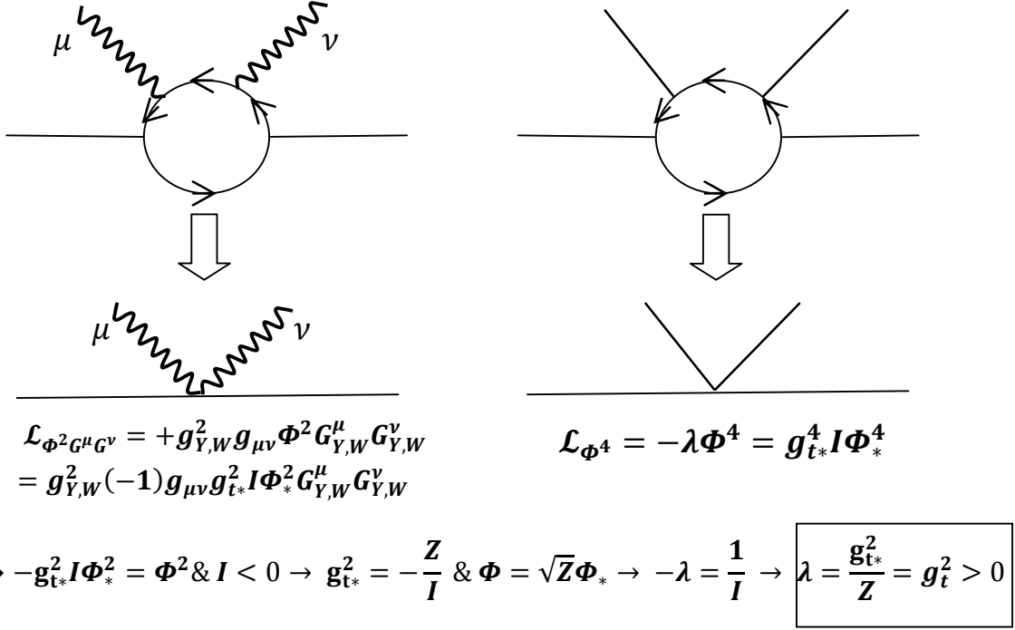
Figure 8 Top loop induced generation of the Higgs scalar electroweak couplings and quartic coupling.
