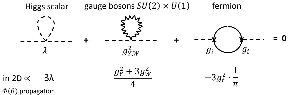
Figure 11 Cancelation of leading quantum corrections for Higgs scalar propagator in 2D Model \pi^{-1/2} .
