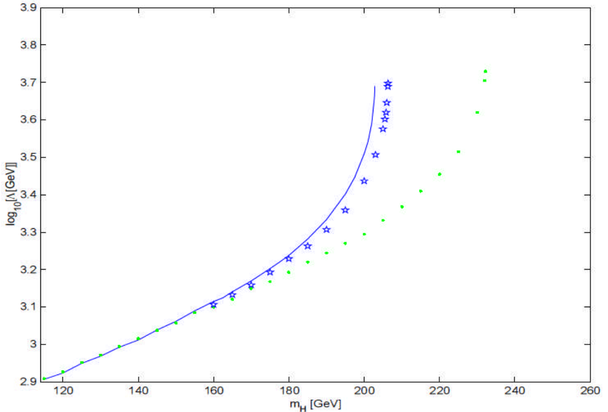
Figure 2 The Higgs Mass Zero Crossing (HMZC) curve as function of the SM physical Higgs mass in the hard-cutoff method (dotted), the \overline{MS} scheme (solid) and with matching as in [61] (pentagrams) [26].
