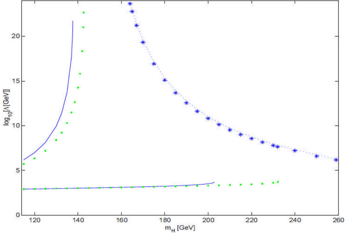
Figure 1 The SM high energy curves as function of the SM Higgs mass [26]. The vacuum stability curve (upper left corner) as obtained in the hard-cutoff method (dotted) and the \overline{MS} scheme (solid). The perturbativity curve (upper right corner) as obtained in the hard-cutoff method (dotted) and the \overline{MS} scheme (solid). The HMZC curve [26] (bottom line), \sim \Lambda_{EWSB} , as obtained in the hard-cutoff method (dotted) and the \overline{MS} scheme (solid).
